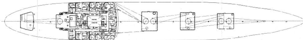
1 st BRIDGE DECK AND TOP OF CRANE HOUSE
